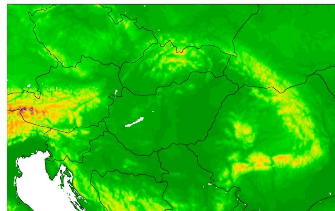
AROME/HU and AROME-EPS domain
