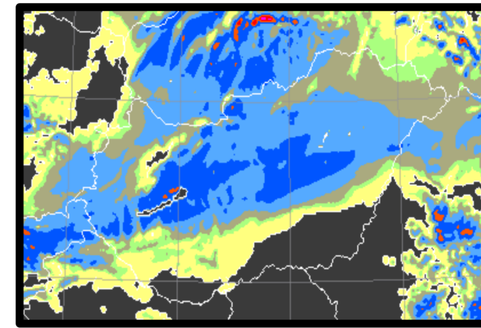
Snow depth [cm] analyses at 6 UTC on 22 November
