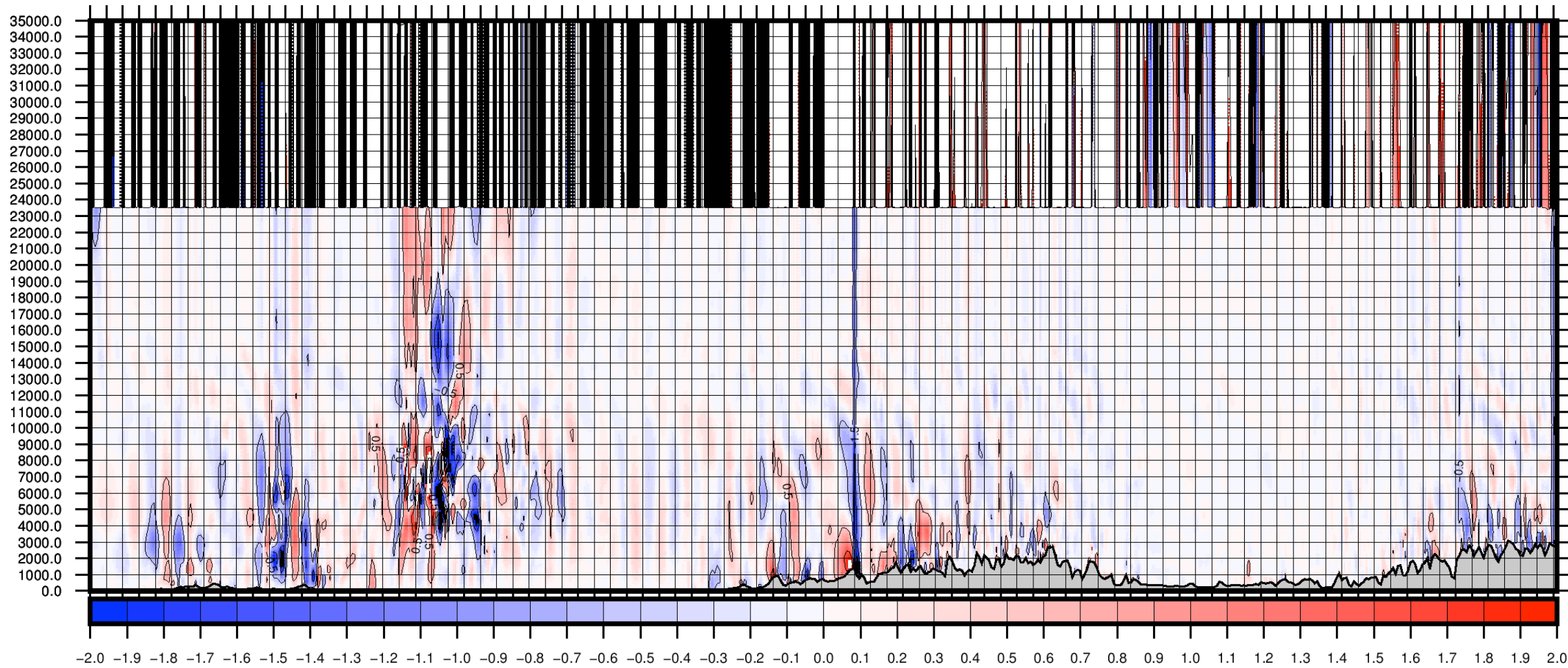
SI SETTLS with new development
