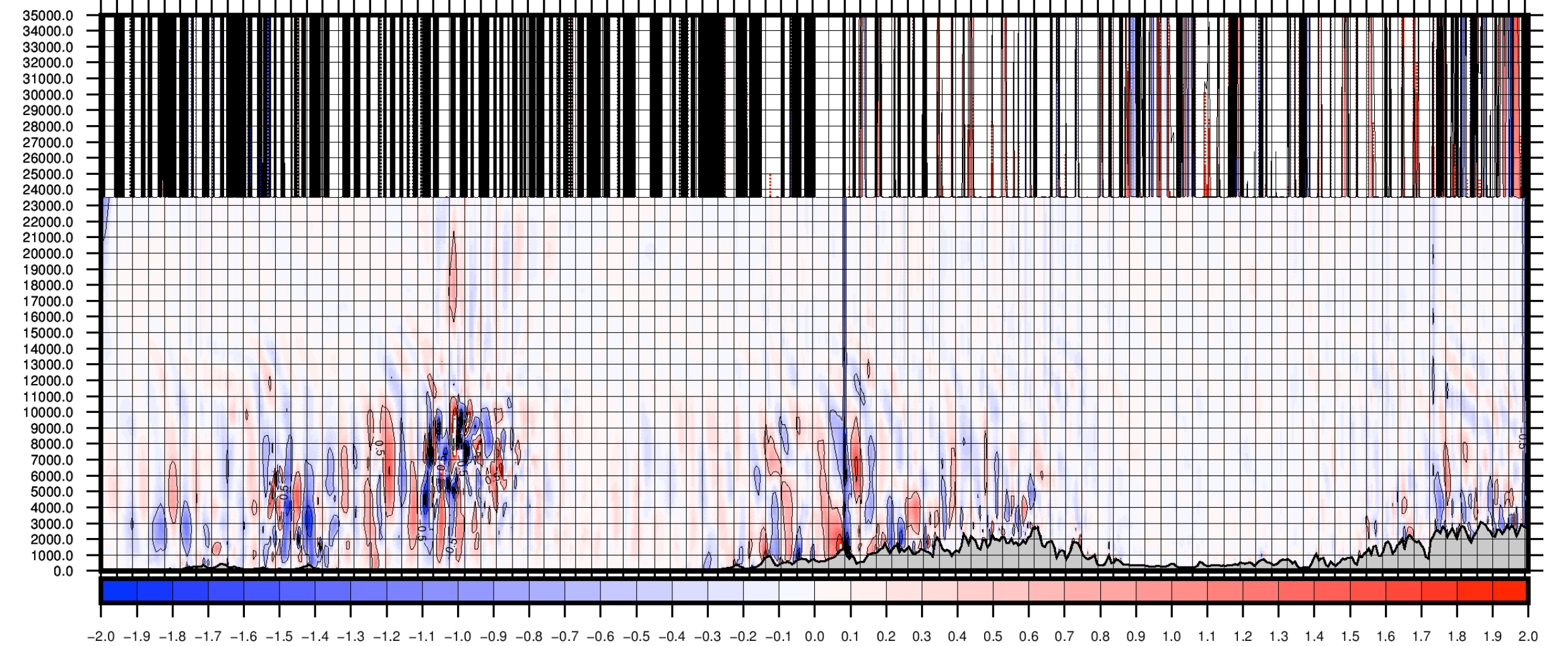
PC CHEAP NESC scheme with NSITER=3
