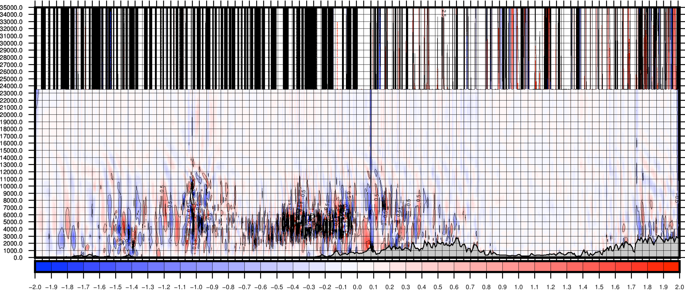
PC CHEAP NESC scheme with NSITER=1
